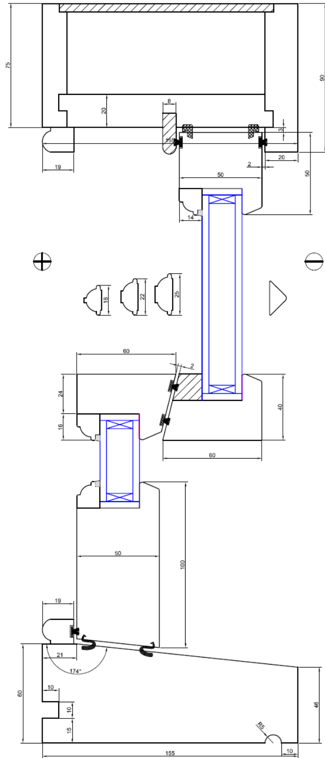
Full box sash window with cords, pulleys and lead weights
